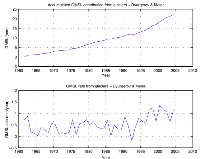
Fig. 5 Contributions from glaciers and ice caps to the global-mean sea level (Dyurgerov and Meier 2005). The lower panel is the annual contribution and the upper panel is the accumulated contribution from 1961
